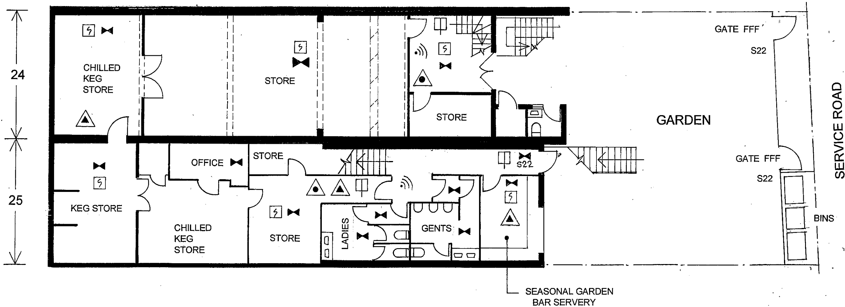
LOWER GROUND FLOOR PLAN @ 1:100
