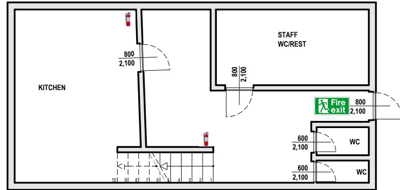
BASEMENT LEVEL Drawing scale 1:100
