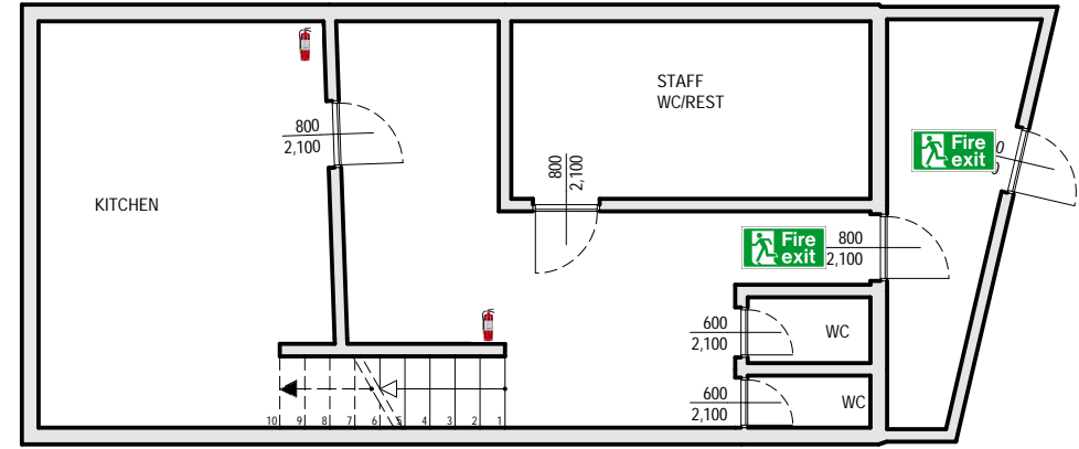
BASEMENT LEVEL Drawing scale 1:100
