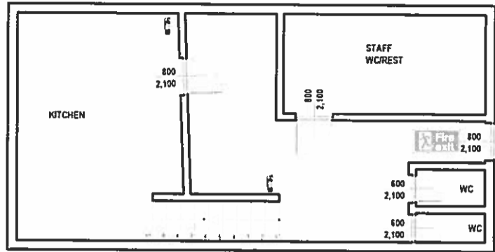
BASEMENT LEVEL Drawing scale 1:100
