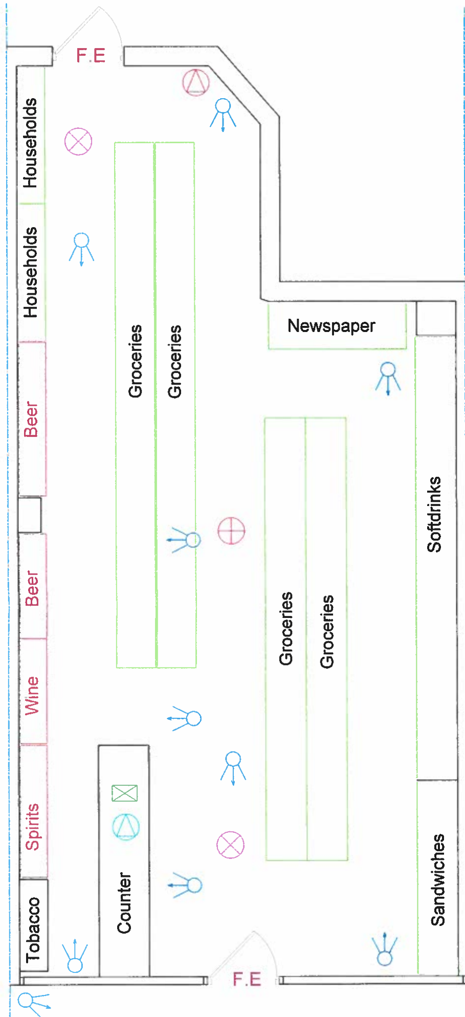
PROPOSED SHOP FLOOR PLAN Scale 1:50
