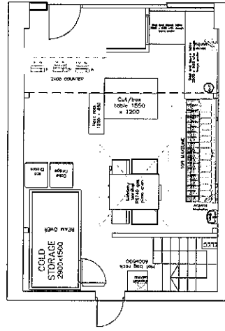
GROUND FLOOR PROPOSED
