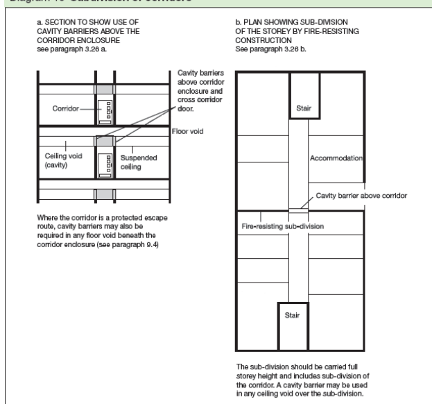
Diagram 16 Subdivision of corridors
