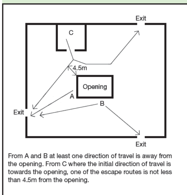
Diagram 14 Open connections
