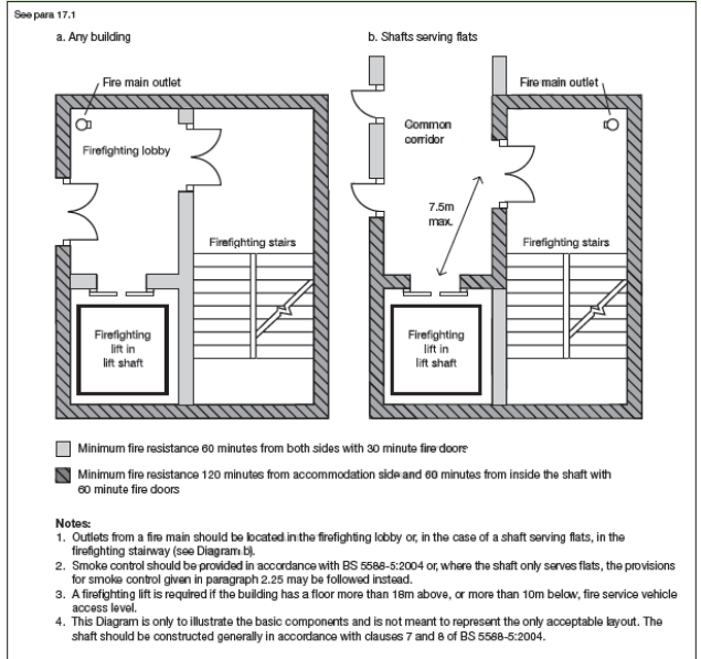
Diagram 52 Components of a firefighting shaft
